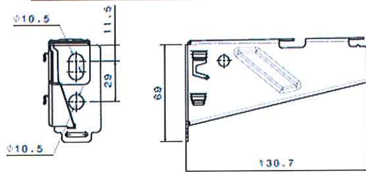
COMPACT BRACKET CB100 Th 1.2 mm
