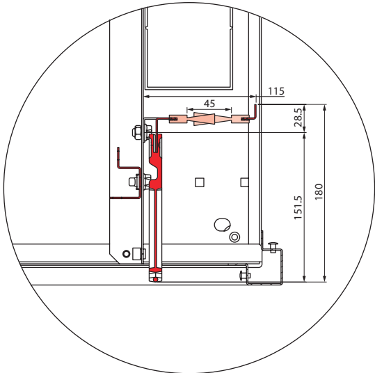
CROSS-SECTION VIEW
