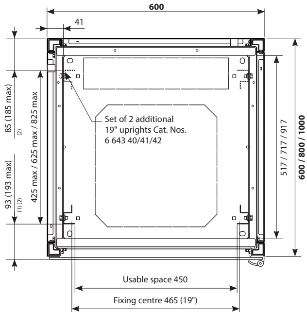
CROSS-SECTION VIEW (3) (with door and side panels)
