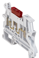
Block Cat. No. 371 80 with blade-type automotive fuse
