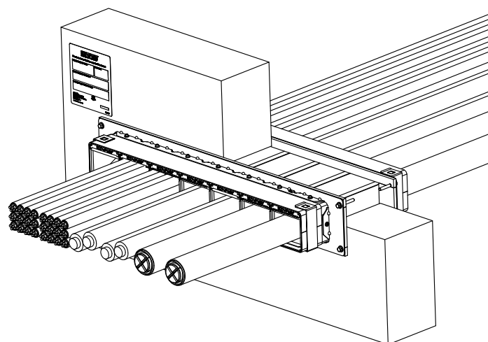
CM250170 + CM250018 (7x) EZF733WT + EZD33T (7x)
